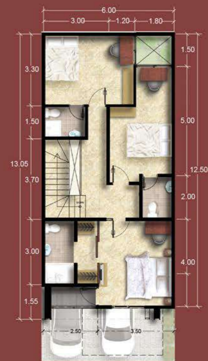
2nd Floor
